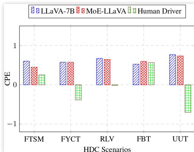
FIGURE 4 CPE Values for Human Driver and VLMs Across HDC Scenarios
