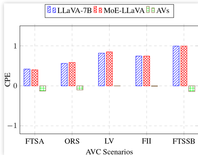
FIGURE 3 CPE Values for AVs and VLMs Across AVC Scenarios
